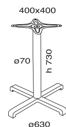
630x630 table base
